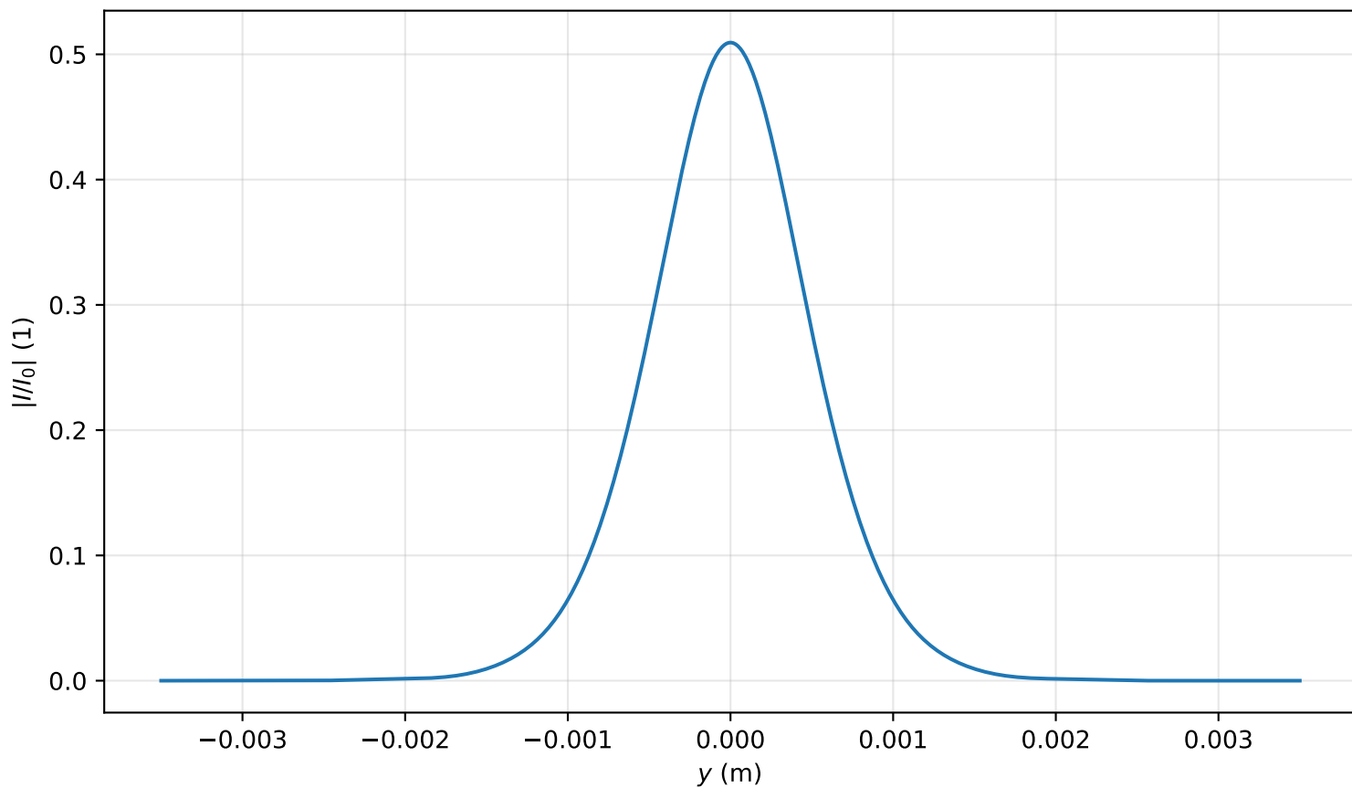
Intensity profile I(x=0, y, z=3.821)/I_0 , P_{in}=0.6P_{cr} , artificial time
